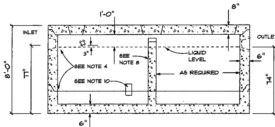
SECTION VIEW
