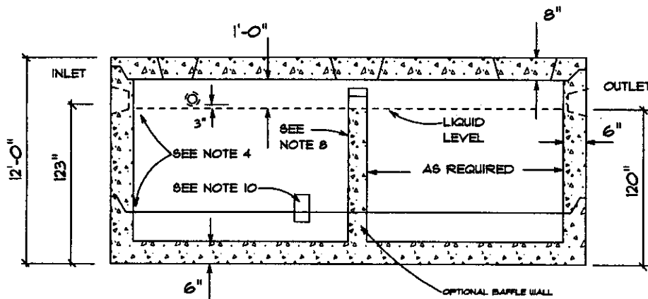
SECTION VIEW
