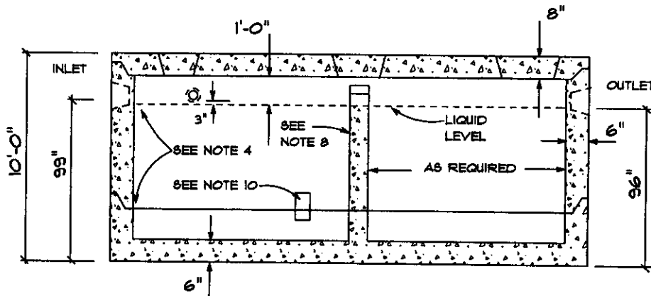
SECTION VIEW
