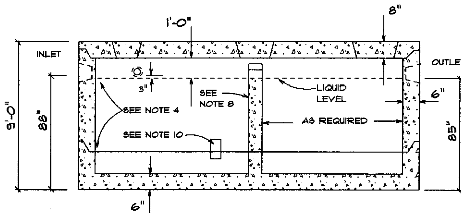
SECTION VIEW
