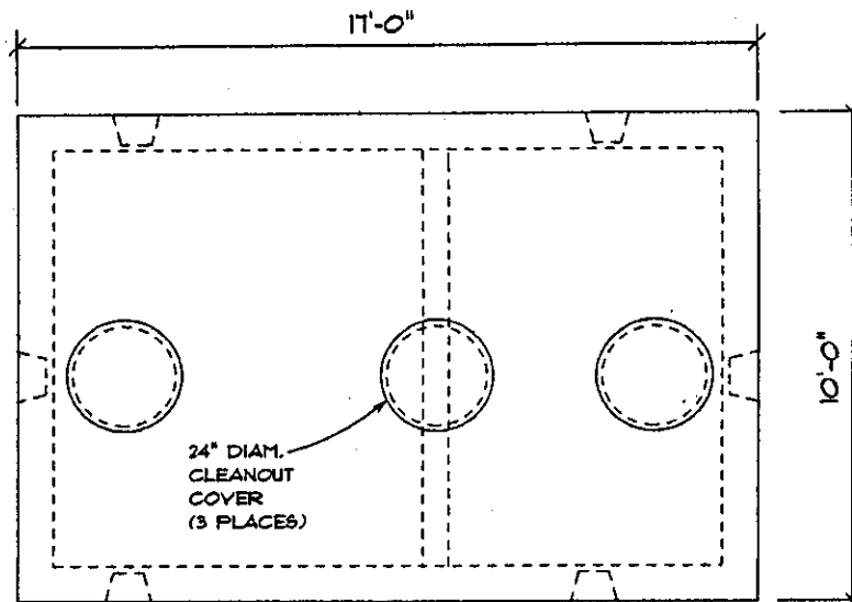
PLAN VIEW
