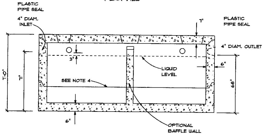
SECTION VIEW
