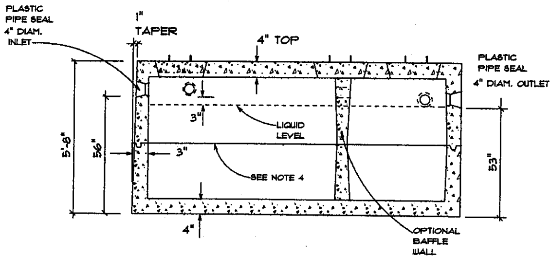
SECTION VIEW
