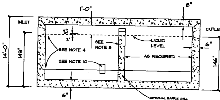
SECTION VIEW
