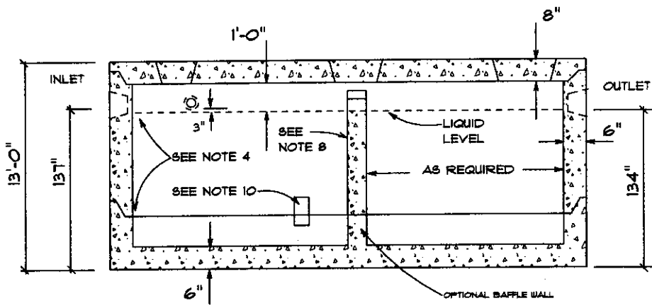
SECTION VIEW
