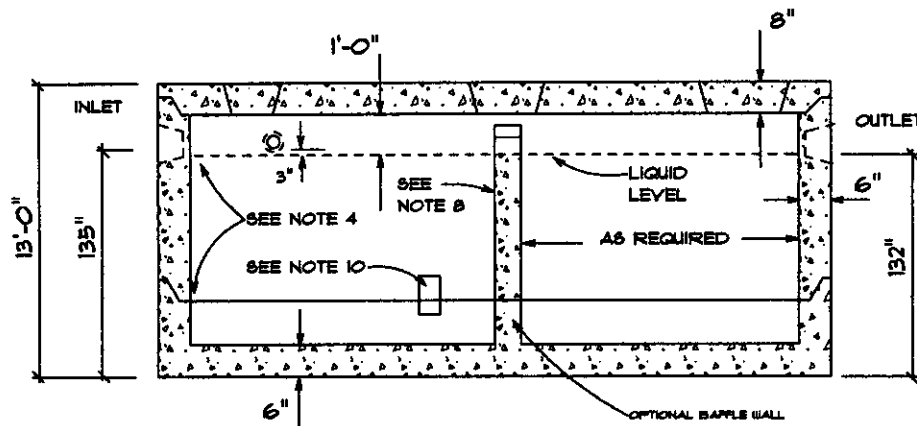
SECTION VIEW
