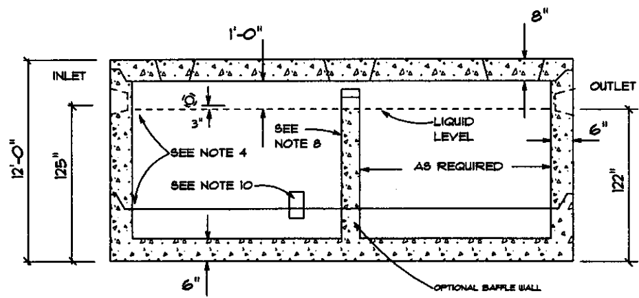
SECTION VIEW
