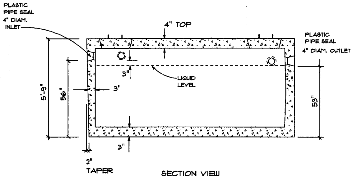
SECTION VIEW
