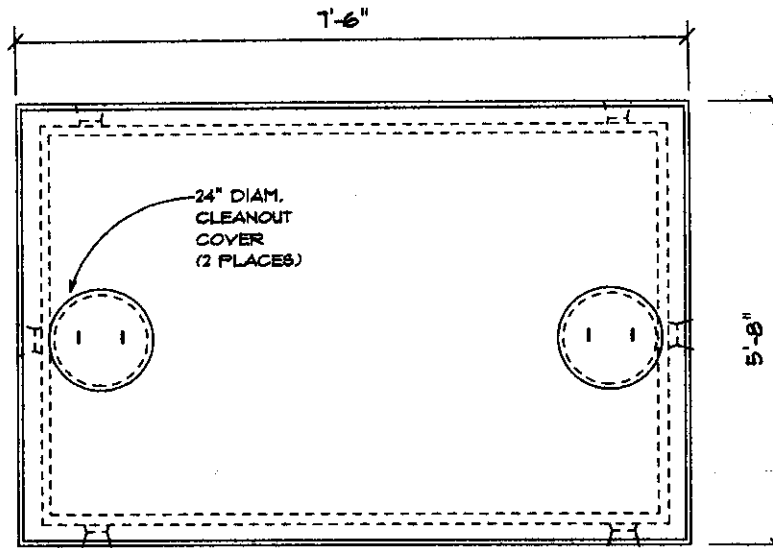
PLAN VIEW
